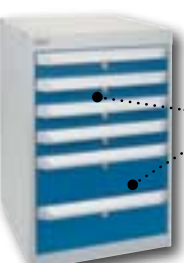
SIX-DRAWER CABINET (4) 15 3/8" W x 20" D x 2 5/8" H (2) 15 3/8" W x 20" D x 5 5/8" H Weight: 94 lbs. Model FH671
